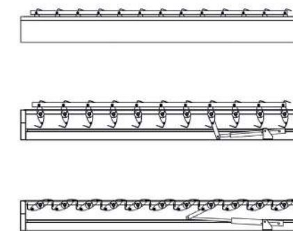
Lateral View PergoLux Without Post
